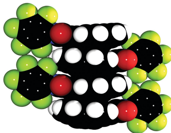
Fig. 3 Space-filling model of the crystal packing in 3a , rendered with POV-Ray. The concave-convex bowl-in-bowl stacking is apparent, while the molecule's orientation and side chains alternate by roughly 180°.
