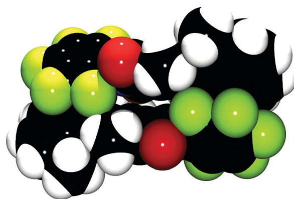
Fig. 2 ORTEP 21 representation (space-filling model) of the crystal packing in 1a , rendered with POV-Ray. 22 The excerpt shows the dense head-to-tail arrangement which proceeds in infinite columns along the crystallographic b axis.
